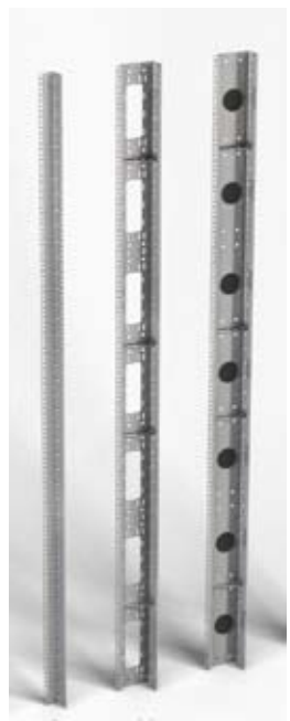
19" extrusions - L, H, C(from the left)
